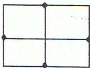
4 odd vertices
